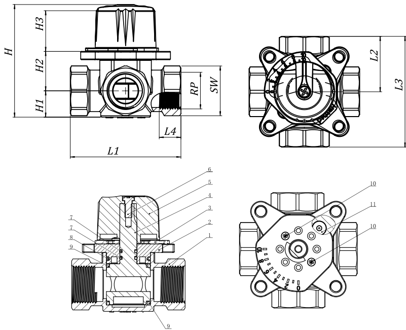
Maßskizze measured sketch
