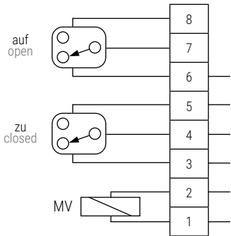
Klemmenplan Wiring diagram
