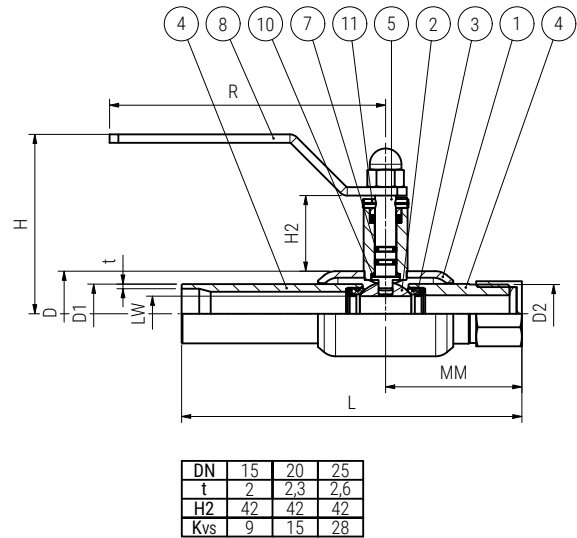
Maßskizze measured sketch
